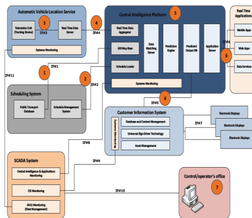
Figure 2: It’s Architecture For Bus Operations
